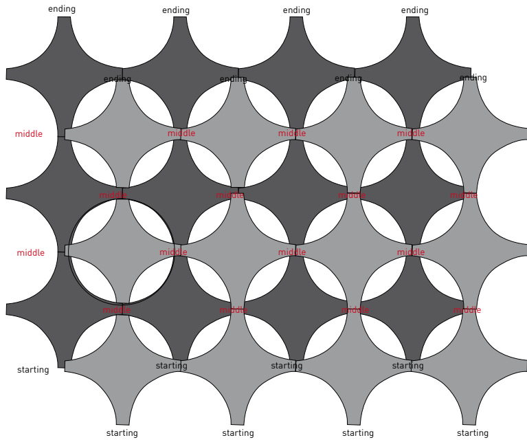
Screw has to allow certain movement to fix the last piece. Ajustar posición grapa para terminar de colocar la pieza
